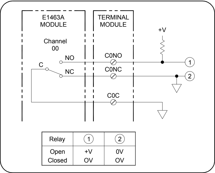
Figure 2-3. Example: Digital Output Configuration
